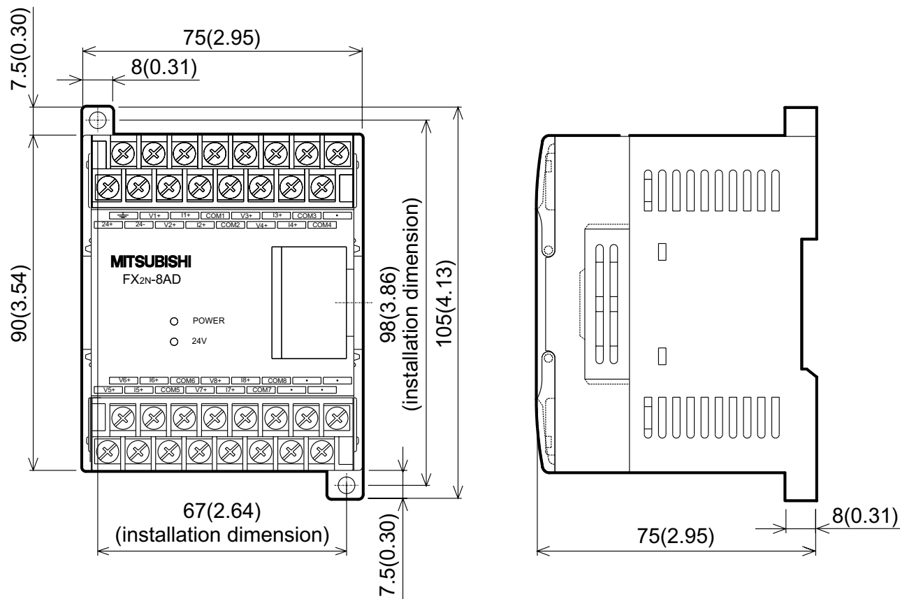
Figure 2.1: External Dimensions
