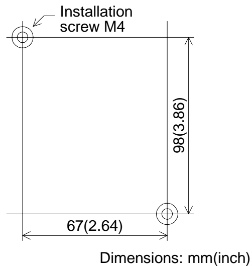
Figure 4.2: Direct installation
