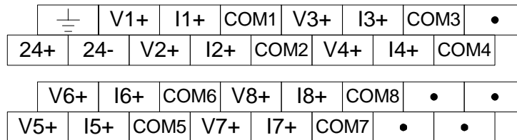
Terminal arrangement
